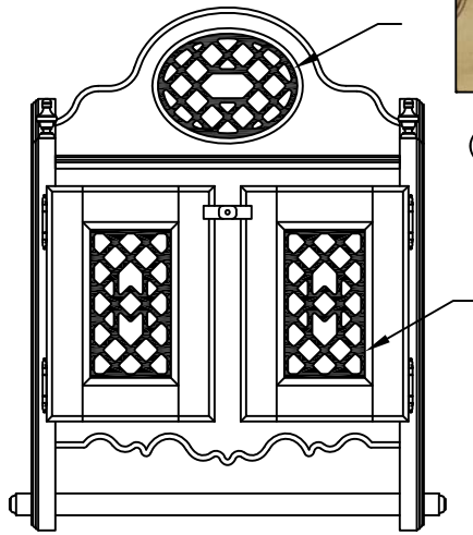
Grillage (S03D-001)
